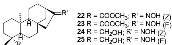
Figure 2. Structures of the synthesized from ent -kauraenoic acid 1 isomeric oximes [31].
