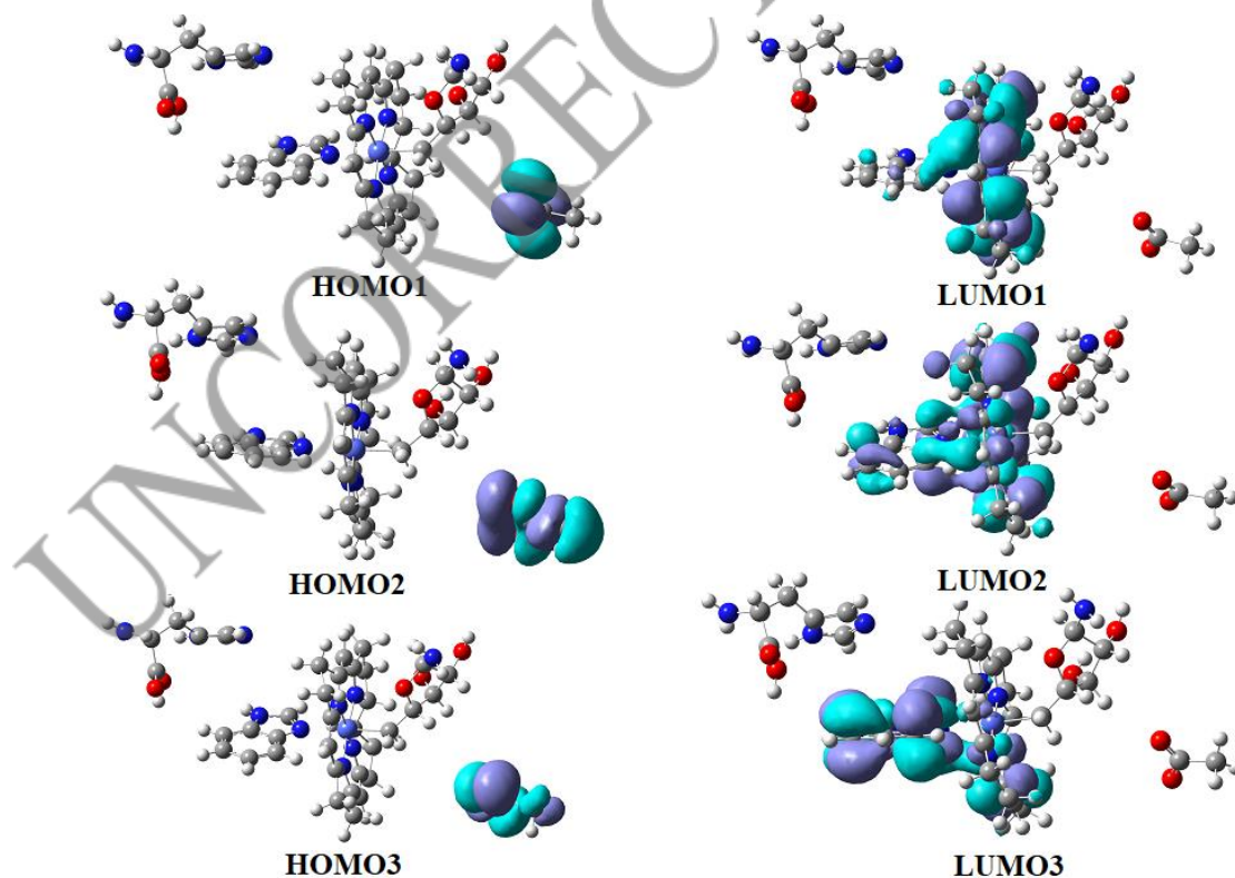
Figure 3. The MCSCF frontier molecular orbital surfaces of the histidine, adenosylcobalamin, and \text{CH}_3\text{COO}^- joint model (Figure 1, see the text).
