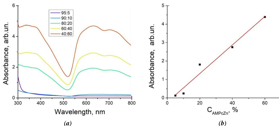
Figure 4. UV-Vis spectra of Chitosan-AmPcZn in DMSO solution (a) and calibration curve showing absorbance as a function of AmPcZn concentration in the copolymer at \lambda = 715 nm (b).
