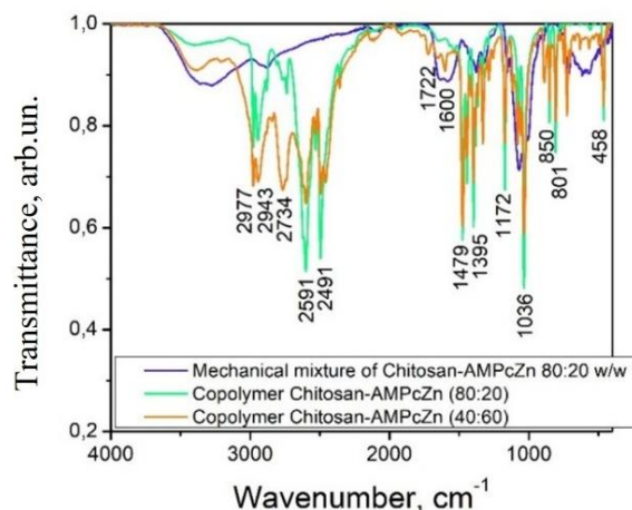
Figure 3. FTIR spectra of the copolymer Chitosan-AmPcZn (80:20) (1), the mechanical mixture of Chitosan-AmPcZn 80:20 w/w (2) and copolymer Chitosan-AmPcZn (40:60) (3).
