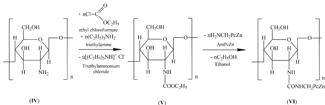
Scheme 2. Grafting of aminomethyl zinc phthalocyanine onto chitosan.
