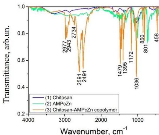
Figure 2. FTIR spectra of Chitosan (1), AmPcZn (2), and the copolymer Chitosan-AmPcZn with ratio 80:20 (3).
