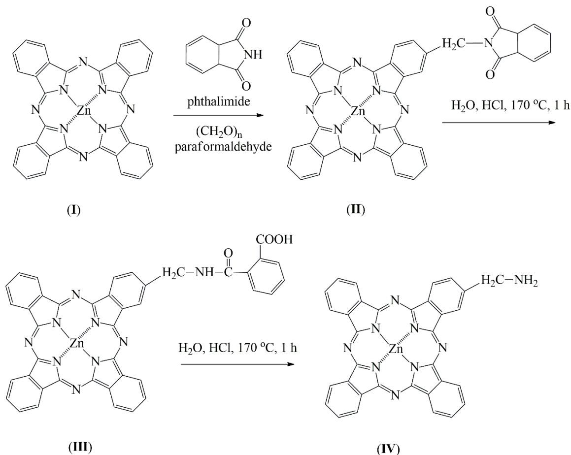
Scheme 1. Synthesis of aminomethyl zinc phthalocyanine.
