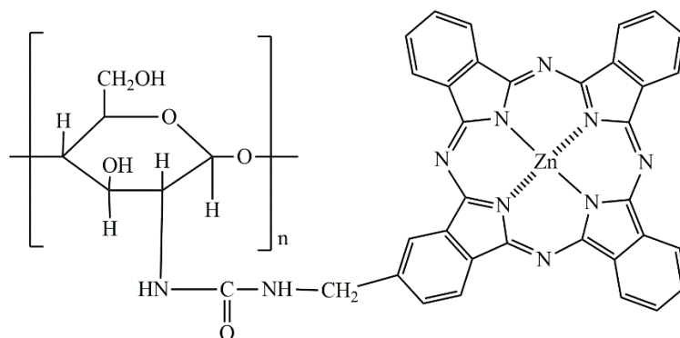
Figure 1. Structural formula of the copolymer Chitosan-AmPcZn.
