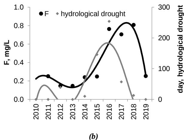
Figure 2. Average concentrations of fluorides in the Dniester river at Camenca station and in Dubasari reservoir, mg/L (a); changes in concentrations of fluorides in Dubasari reservoir as a function of the number of days of hydrological drought (b).
